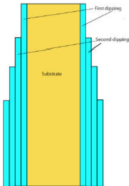
FIGURE 1.7.2 Staircase on both sides of a glass slide by repetitive Langmuir-Blodgett deposition.
