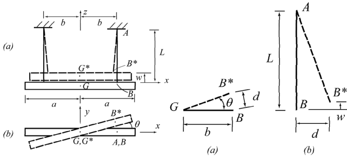
Figure 2 Deformation geometry.
